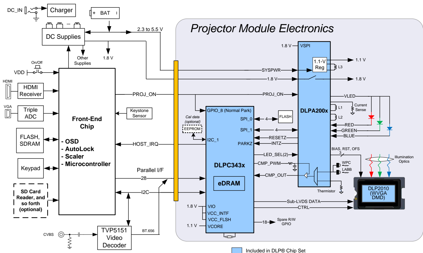
Figure 1. DLPC343x System Configuration
